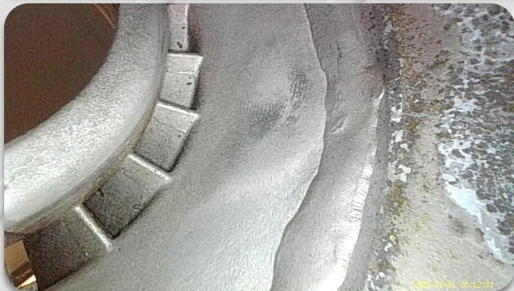
Burner Can Inspection with 6mm HXVB6015
